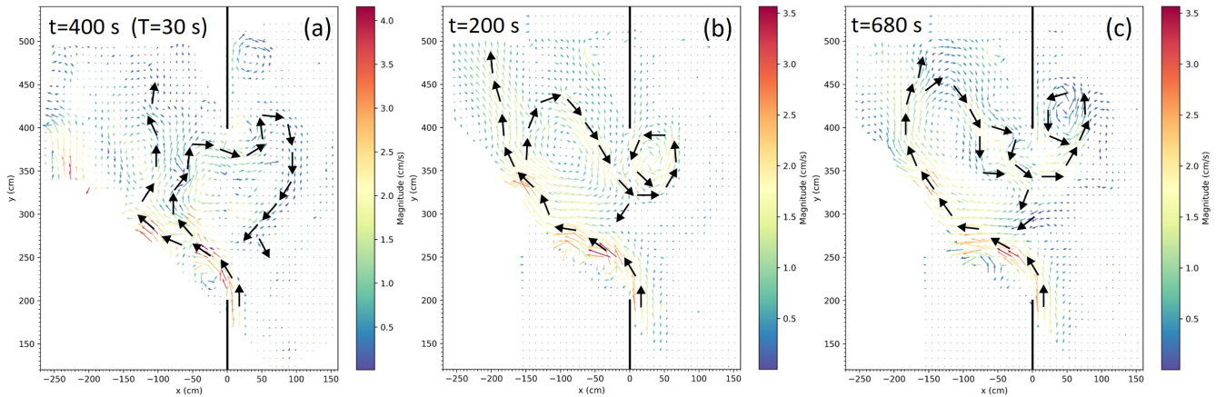
Figure 8. (a): Snapshot of the current velocity field (in \text{cm s}^{-1} ) at t = 400 \text{ s} for Q = 2 and T = 30 \text{ s} (cf. Supplementary Figures S3-S5). (b,c): same but for T = 60 \text{ s} at t = 200 \text{ s} and at t = 680 \text{ s} , respectively.
