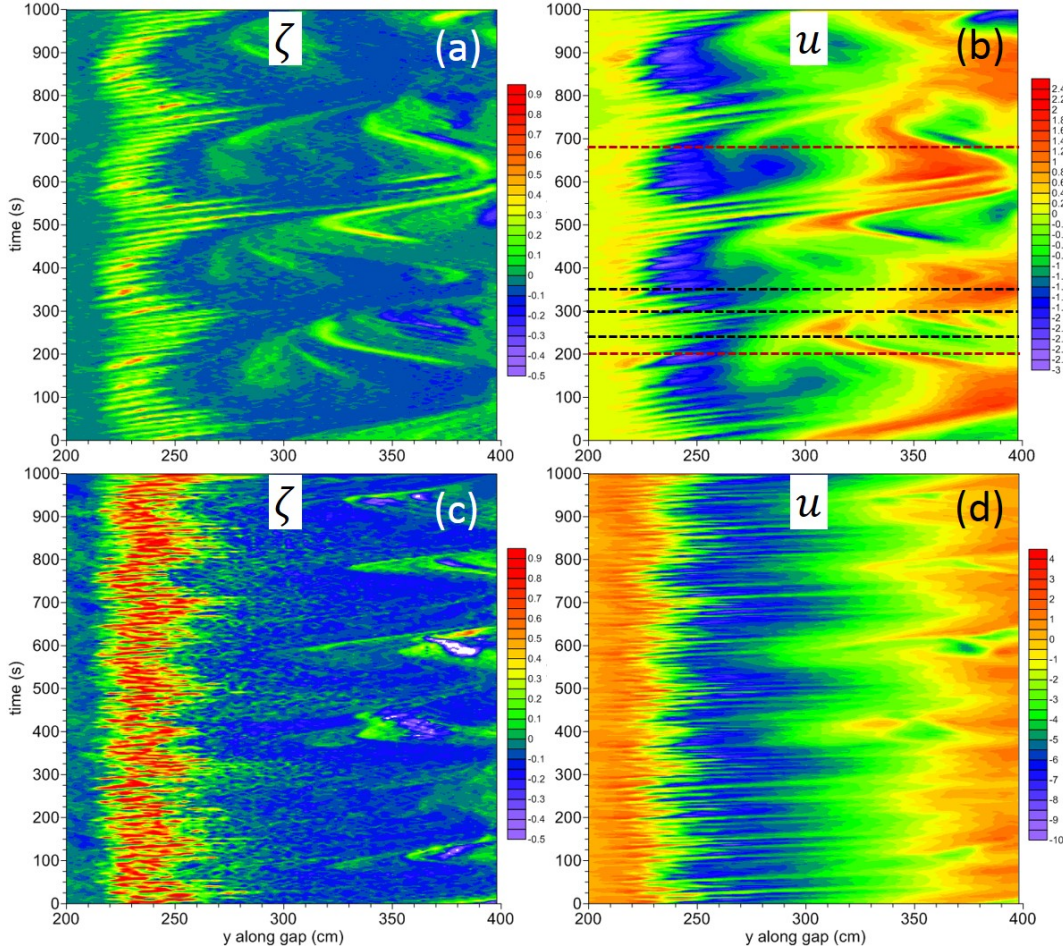
Figure 6. Hovmöller diagram of the relative vorticity \zeta (in s^{-1} ) –panel (a)– and current velocity u (in cm\ s^{-1} ) –panel (b)– for a rotation period T = 60\ s and Q = 2 . Panels (c,d): same but with Q = 8 . The velocity profiles of u along the black dashed lines in panel (b) are shown in the Supplementary Figure S6 and the corresponding snapshots of the 2D \mathbf{u} –field are shown in Fig 7. The brown dashed lines in panel (b) correspond to the snapshots of Figs. 8(b,c).
