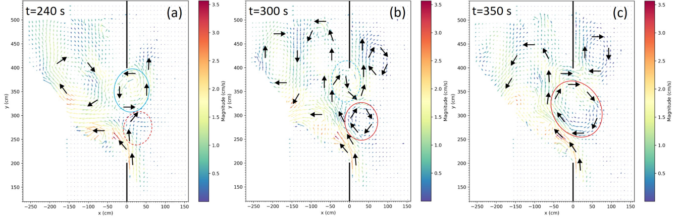
Figure 7. Snapshots of the current velocity field (in \text{cm s}^{-1} ) at t = 240 \text{ s} (a), t = 300 \text{ s} (b) and t = 350 \text{ s} (c) for Q = 2 and a rotation period T = 60 \text{ s} (see the black dots in Fig. 5(a), the u -field along black the dashed lines in Fig. 6(b) and Supplementary Figure S6 for the u -profiles along the gap).
