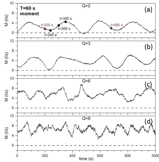
Figure 5. Time series of the moment M (in \text{litres s}^{-1} ) for different values of Q (2, 3, 6, 8) and for a rotation period T = 60 \text{ s} .
